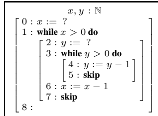
Fig. 5. Program NESTED-LOOPS
