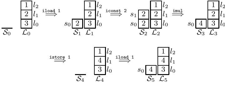
Fig. 2. Stack and local variables during an execution of some bytecodes.
