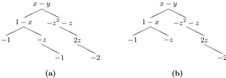
Fig. 2. (a) Finite difference tree for CHASE of x - y with respect to \{\tau_1, \tau_2\} . (b) Tailored finite difference tree.
