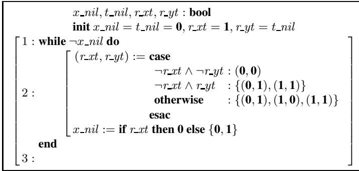
Fig. 3. Program ABSTRACT-LIST-REVERSAL
