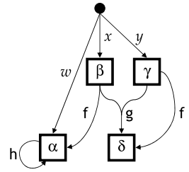
Fig. 4. An e-graph.
